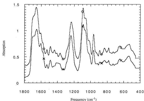
FIG. 5. MIR absorption spectrum of wet-spun films of NaDNA-netropsin (○) and NaDNA (×) at low RH.
