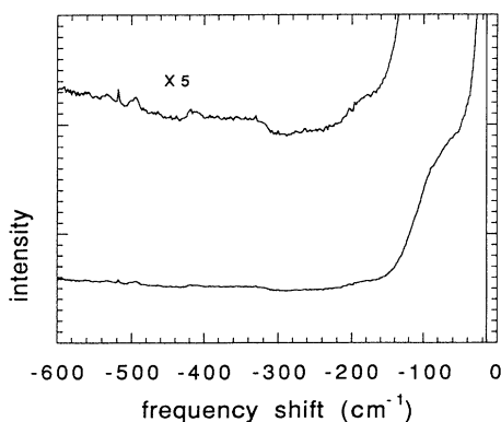
FIG. 3. The low-frequency Raman spectrum from a wet-spun film of NaDNA-netropsin at 75% RH.
